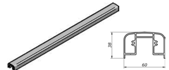
Profilo corrimano lungh. 5000 argento Handrail profile length. 5000 silver
