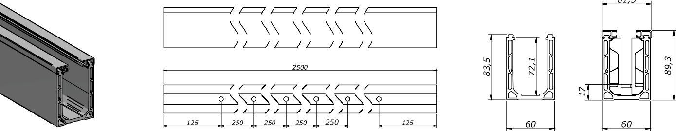
Profilo di supporto Sirio Small pre-forato lungh. mm 2500 Sirio Small U-channel base profile pre-drilled length mm 2500
