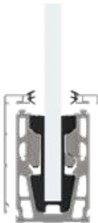
carter laterale + superiore / side + top cover
