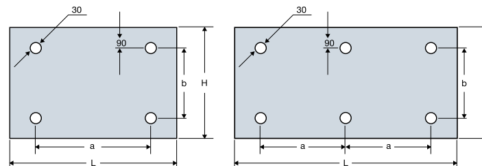
Lastre con 4 fori Glass with 4 holes
